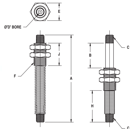
Spring Leveler Groups 2 & 3
