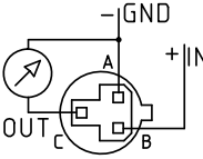
B (IN) C (OUT) A (GND)
